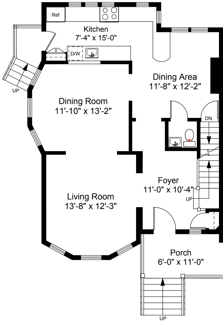
First Floor Plan Ceiling Height = 8'-5"
