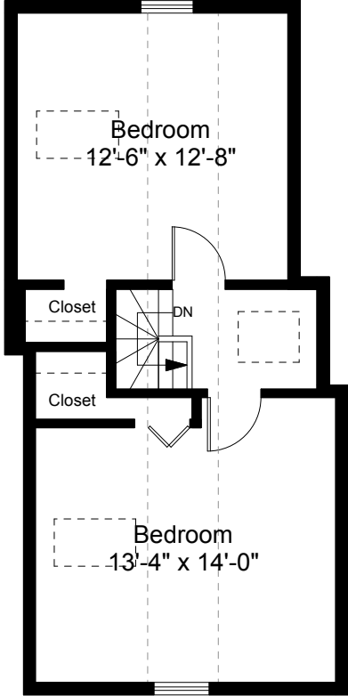
Third Floor Plan Ceiling Height = 8'-6"
