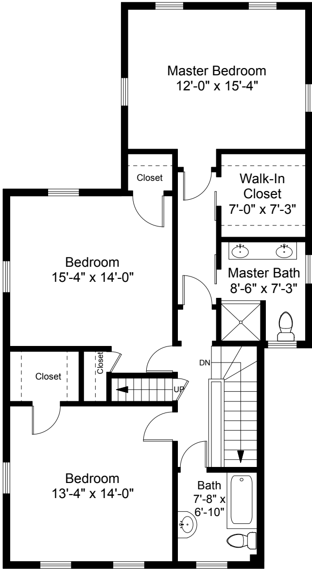
Second Floor Plan Ceiling Height = 8'-6"
