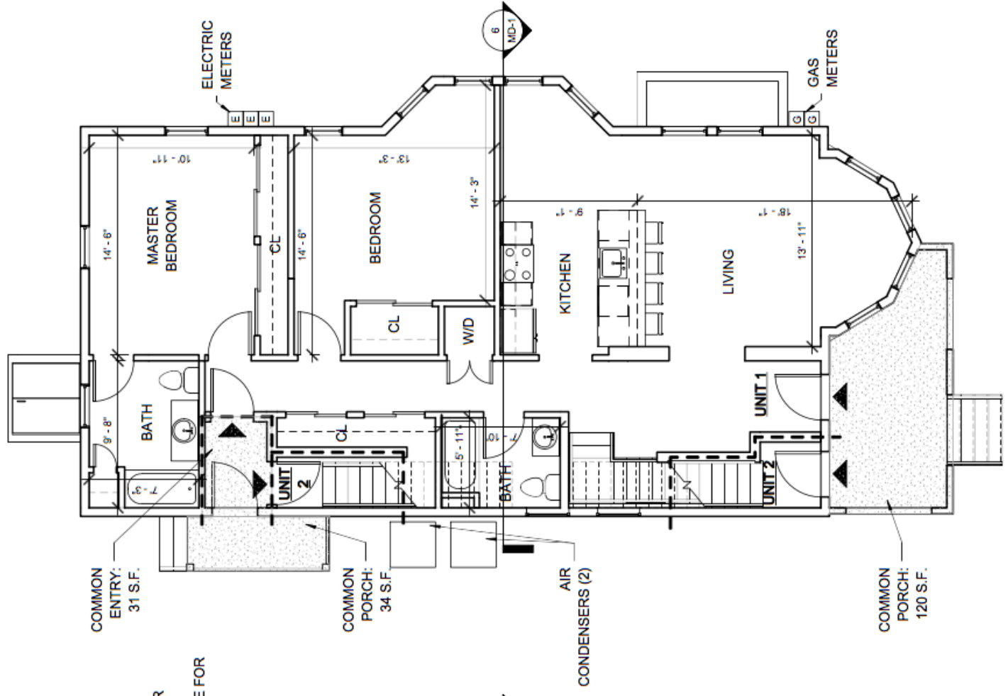
② First Floor 3/16" = 1'-0"
