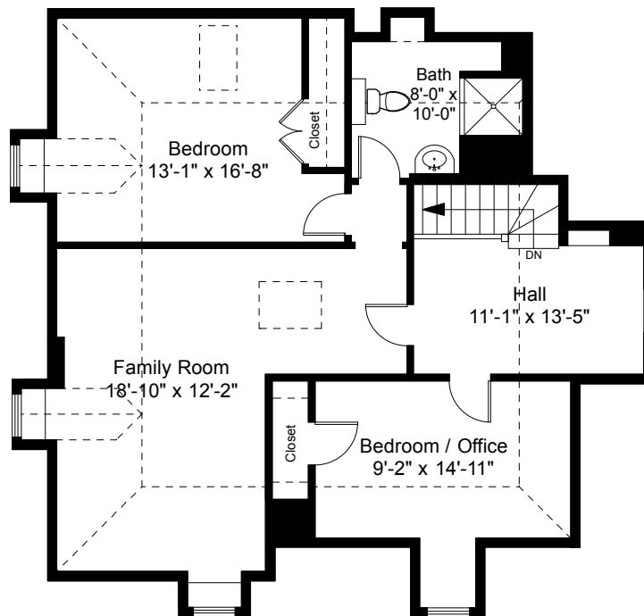
Third Floor Plan Ceiling Height = 8'-0"
