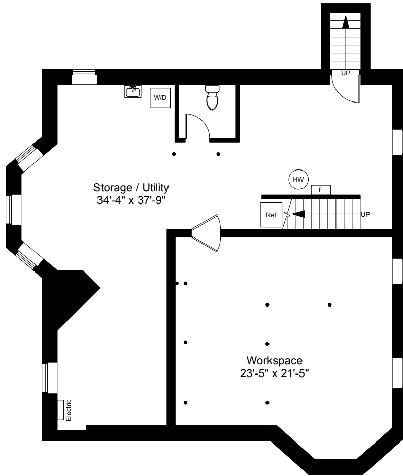
Basement Plan Ceiling Height = 7'-5"
