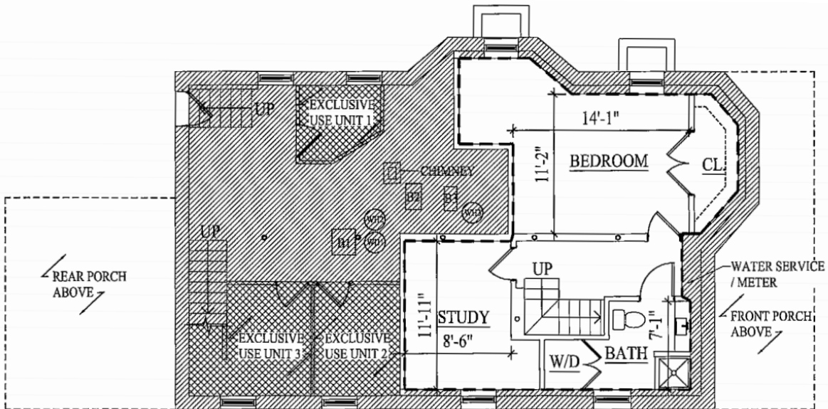
BASEMENT LEVEL PLAN - UNIT 1 (LOWER LEVEL)
