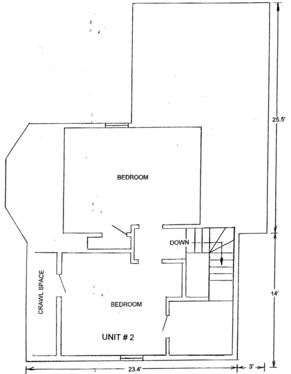
THIRD FLOOR
