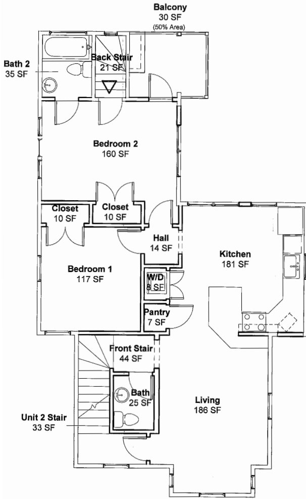
③ Unit 2 (Floor Two) 3/16" = 1'-0"
